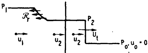
(c) PRESSURE-DISTANCE PROFILE AFTER INTERACTION
